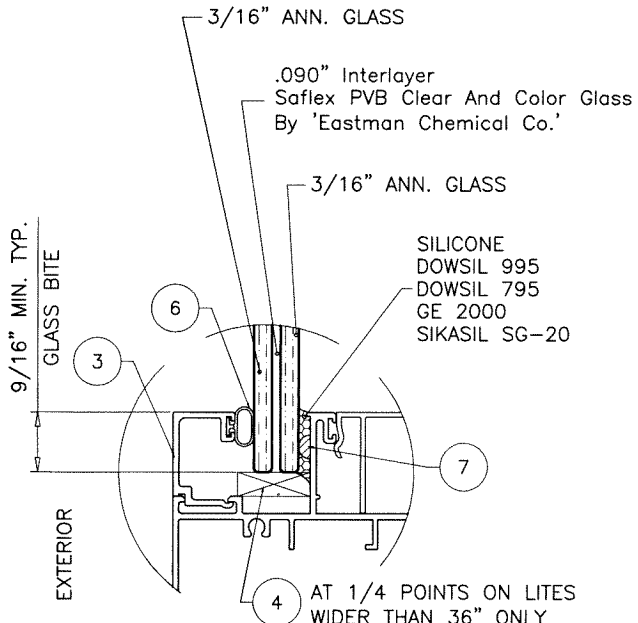
GLASS TYPE 'A' 7/16" OVERALL LAM. GLASS
